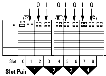
Primary Chassis
